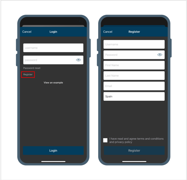
Figure 3. Login screen
