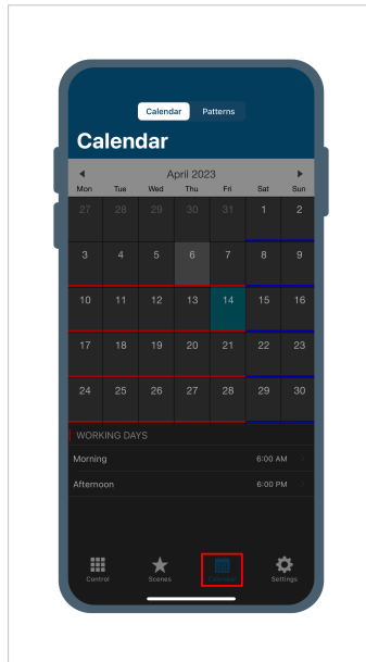
Figure 9. Calendar menu
