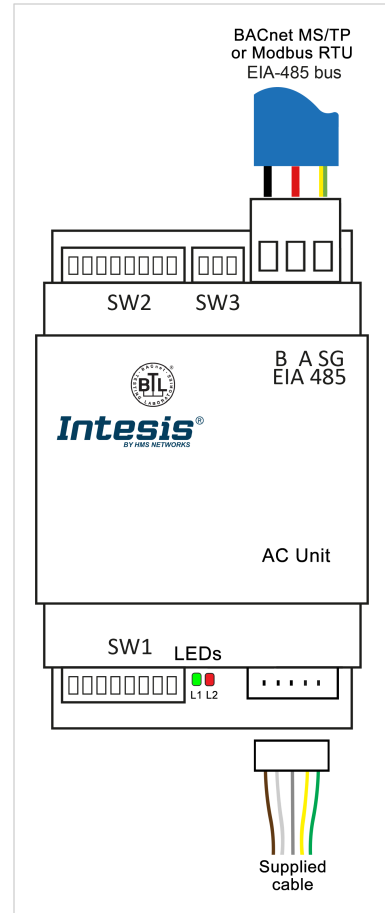
Figure 1. Wiring diagram (wire colors are indicative only)
