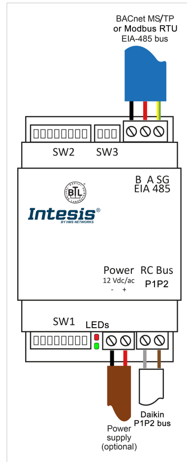
Figure 1. Wiring diagram (wire colors are indicative only)
